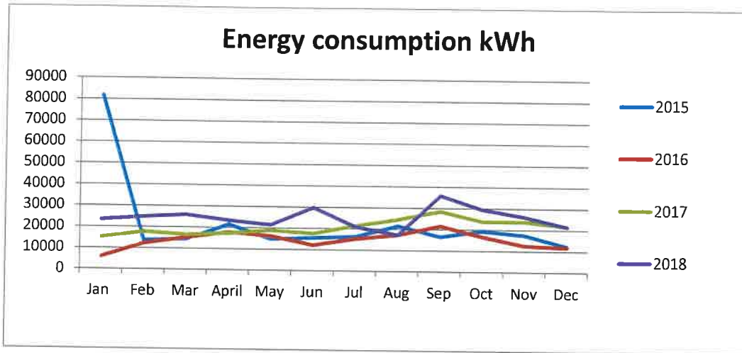
Figure 1: Year-wise monthly energy consumption pattern
